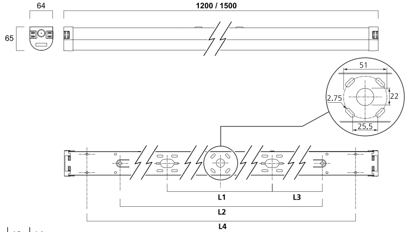
START Batten 1200/1500
